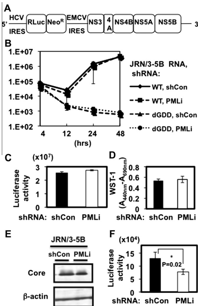
Fig. 2. PML is unrelated to the HCV RNA replication. Schematic gene organization of subgenomic JFH1 (JRN/3-5B) RNA encoding Renilla luciferase (RL) gene. Renilla luciferase gene (RLuc) is depicted as a box and is expressed as a fusion protein with Neo. (B) The transient replication of subgenomic HCV-JFH1 replicon in the PML knockdown (PMLi) or the control OR6c cells (shCon) after electroporation of in vitro transcribed JRN/3-5B RNA (10 \mu g) was monitored by RL assay at the indicated time. The results of Renilla luciferase activity are shown. dGDD indicates the deletion of the GDD motif in the NS5B polymerase, and the subgenomic HCV replicon with the deletion of GDD was used as a negative control. (C) The level of HCV RNA replication in PML knockdown (PMLi) or the control (shCon) OR6c JRN/3-5B cells was monitored by RL assay. The results shown are means from three independent experiments. (D) WST-1 assay of the PML knockdown or the control JRN/3-5B cells. (E) The level of HCV core protein in OR6c JRN/3-5B cells by expression of HCV core to NS2 coding region of HCV-JFH1 using mouse retroviral vector. pCX4bsr-JFH1-myc-C-NS2 and pMDG2 were cotransfected into Plat-E cells, mouse retroviral packaging cells. Mouse retroviral vector was obtained from their culture supernatants and transduced into OR6c JRN/3-5B PML knockdown or the control cells. The results of Western blot analysis of cellular lysates with anti-HCV core or an anti \beta -actin antibody are shown. (F) The level of HCV RNA replication in RSc cells 72 h after inoculation of HCV-like particles produced using trans -packaging system was monitored by RL assay. Asterisk indicates significant difference compared to the control. *P = 0.02.
